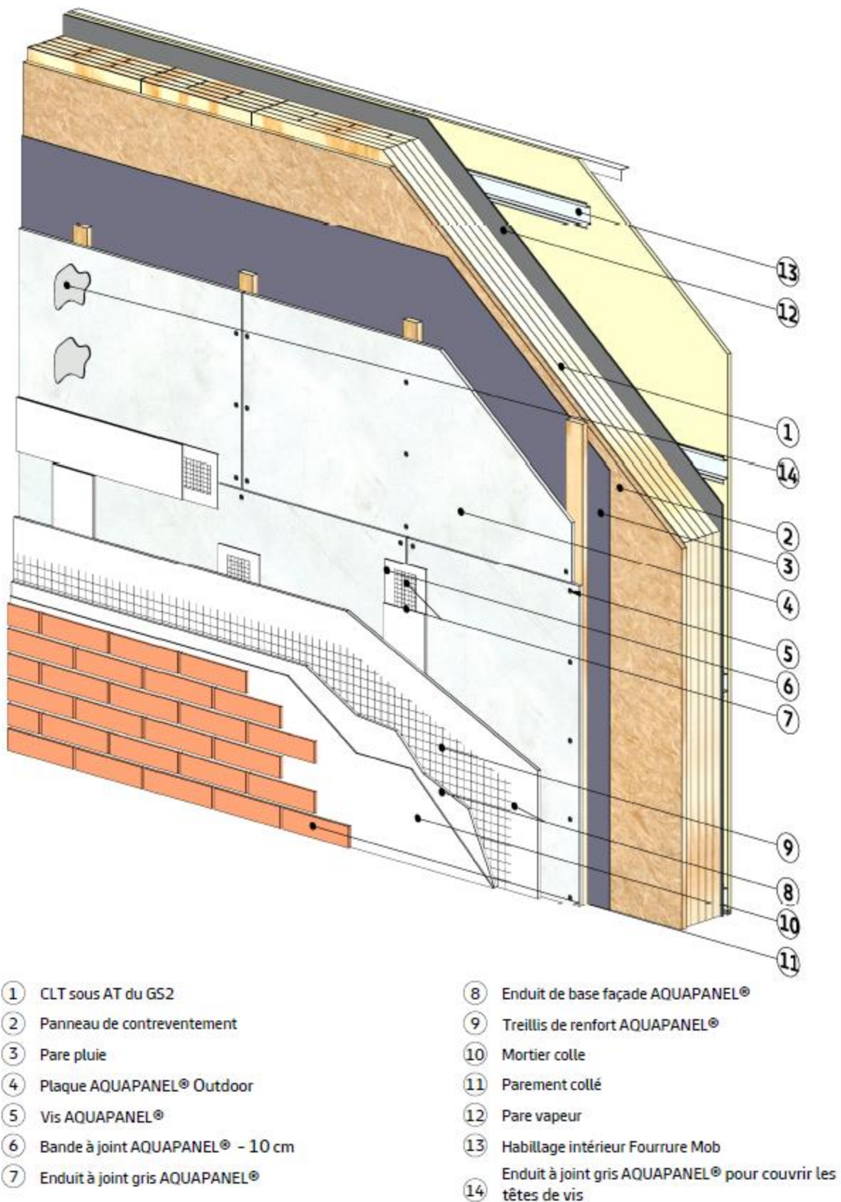
Figure 3 - Principe Bardage Aquapanel sur tasseaux - support CLT
